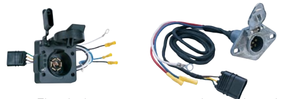
Electrical connectors commonly used in towing
